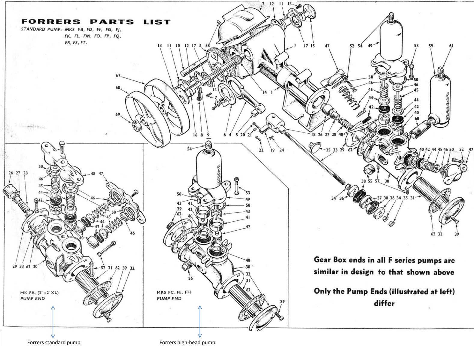
Forrers standard pump
