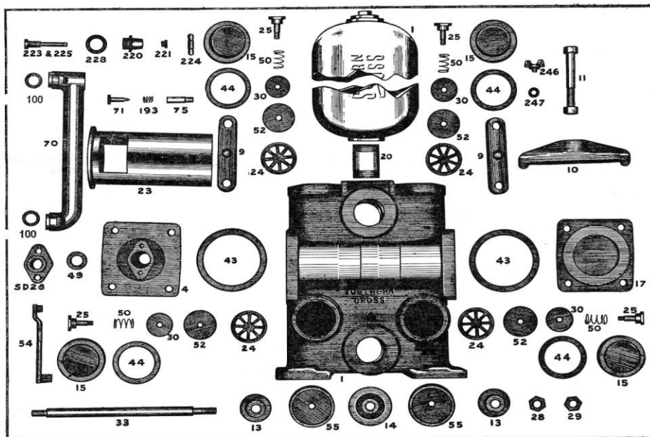
Marks AN-I, AN-K and AN-L Power Pump Parts
